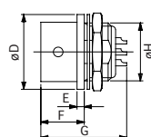
Bulkhead Mount Receptacle
